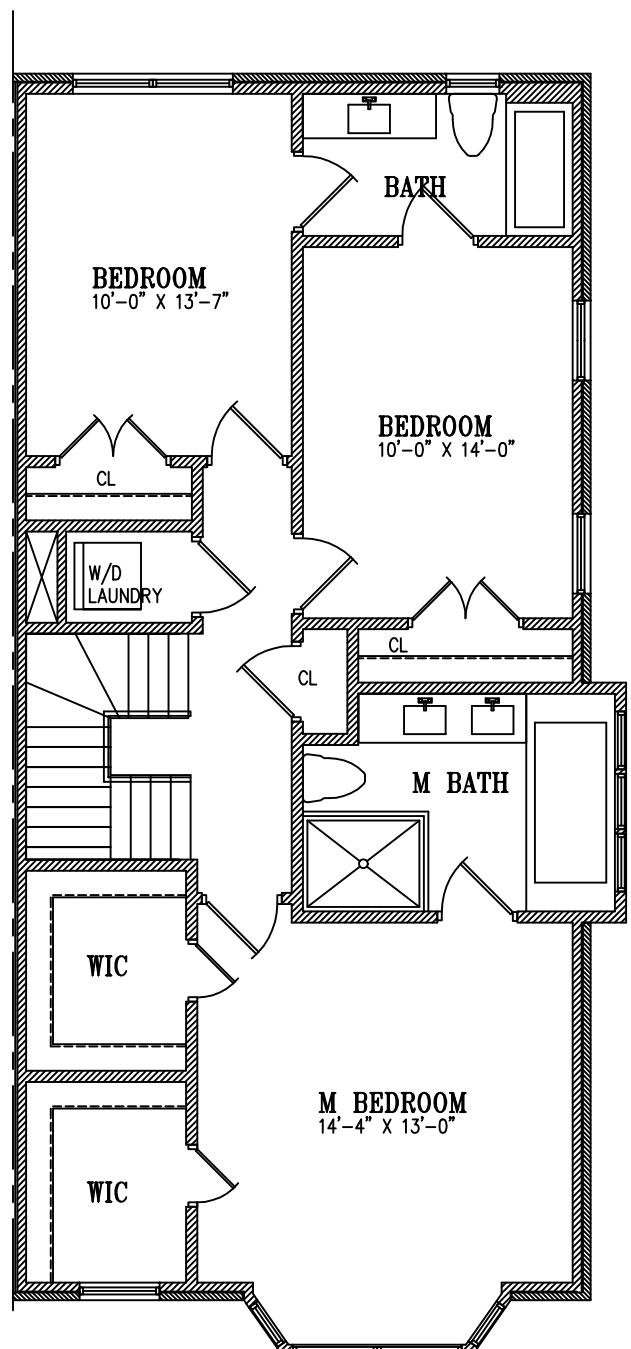
SECOND FLOOR PLAN UNIT A
