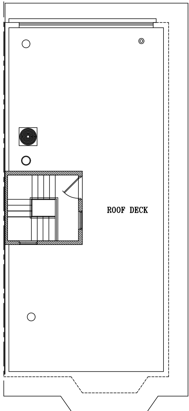
ROOF FLOOR PLAN UNIT A
