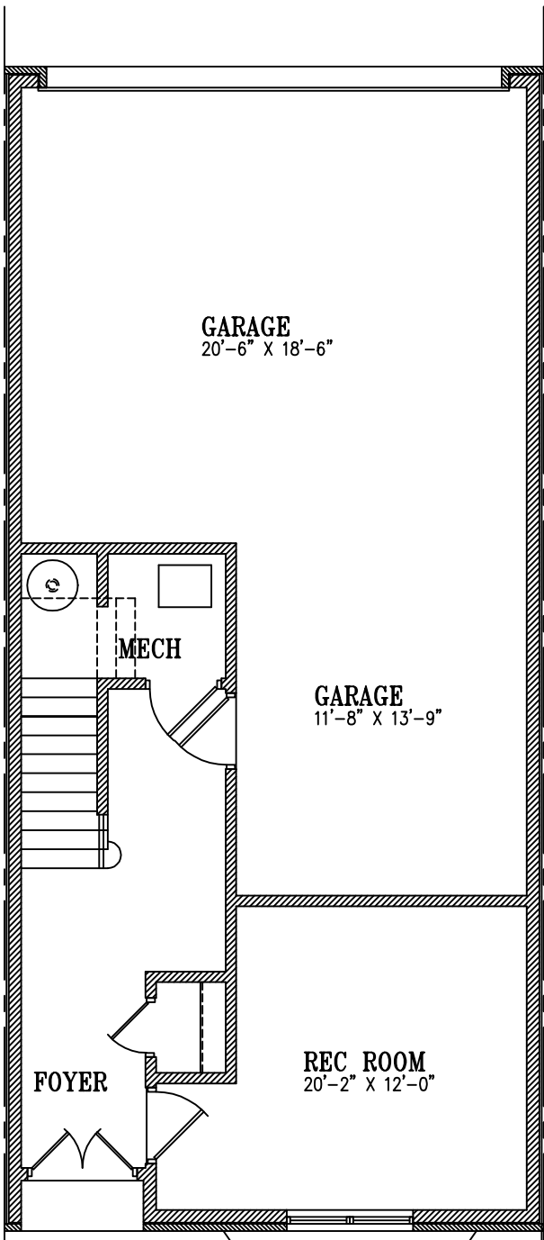
FLOOR PLAN LOWER LEVEL UNIT C
