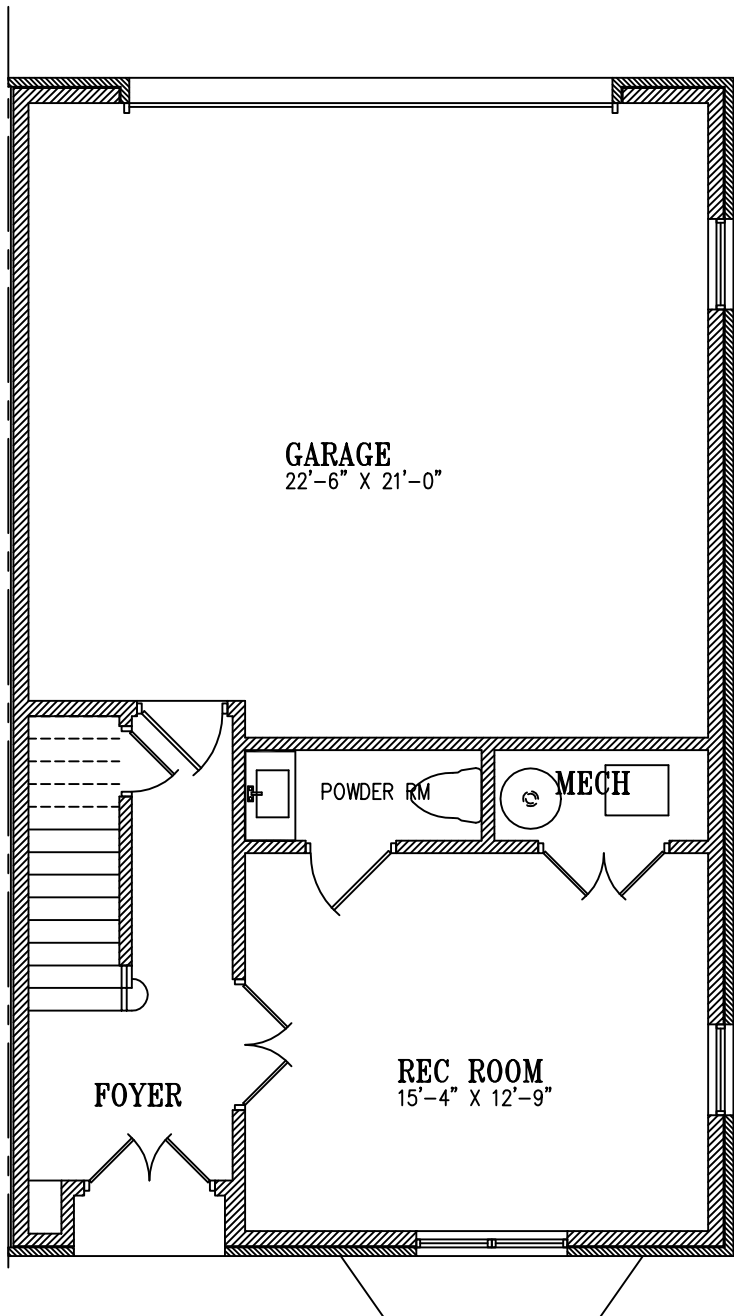
FLOOR PLAN LOWER LEVEL UNIT D
