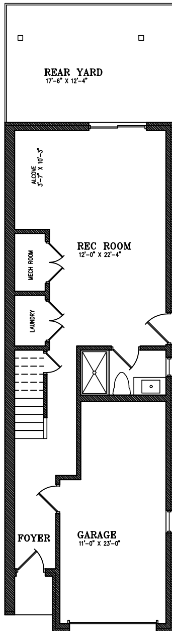
GROUND LEVEL PLAN 910 SF
